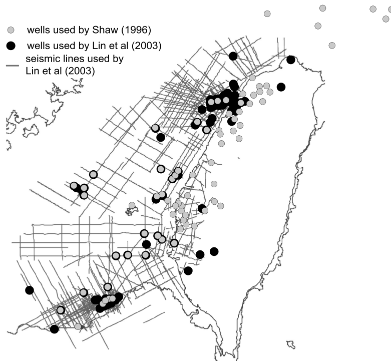
Figure 4. Seismic lines and well coverage used in the study of Lin et al. [2003] to define the geometry of the foreland basement shown on Figure 3. The isopach maps of the synorogenic sediments of Figure 5 were derived by Shaw [1996] essentially based on well logs. In any case the total foreland thicknesses by Shaw [1996] were consistent with the depth to basement proposed by Lin et al. [2003].
