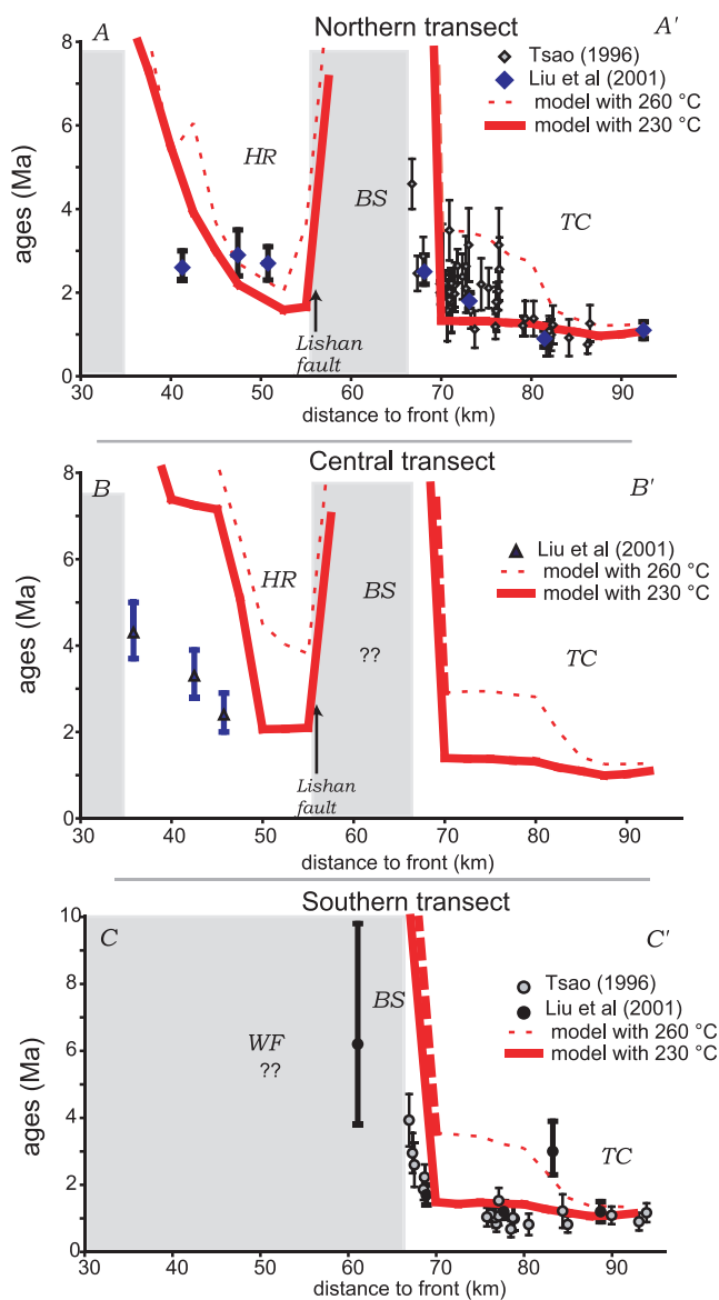
Figure 9. FT ages on detrital zircon from Liu et al. [2001] and Tsao [1996] with 2\text{-}\sigma error bars and predictions from our thermokinematic model by assuming a closure temperature of 260^\circ\text{C} (dashed red line) and 230^\circ\text{C} (solid red line). Pooled ages are taken for the data from Tsao [1996]. In the case of the data from Liu et al. [2001], \chi^2 ages are considered. Shaded areas indicate where the ages are partially reset or nonreset. In the case of the central transect, no data are available for the BS and TC, and we assume that the extent of the area where ages are not reset is similar to that of the northern transect. Also data are not available over the WF of the southern transect, and we suppose that ages may be not reset or only partially reset.
