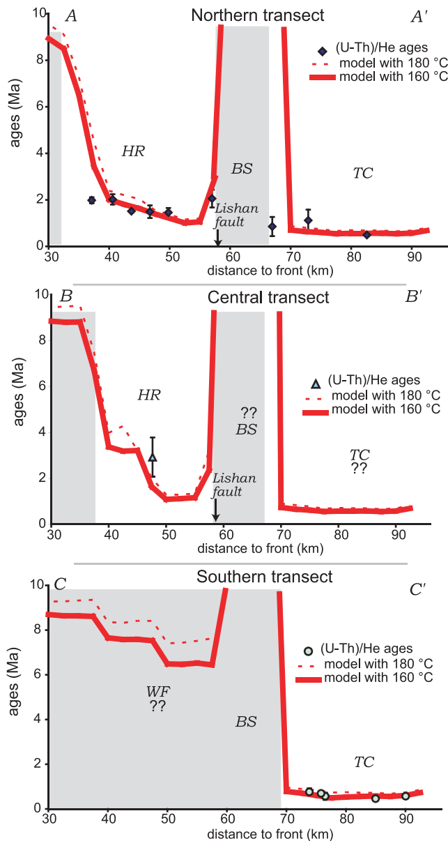
Figure 10. (U-Th)/He ages on detrital zircon [Beysac et al. , 2007] with 2\text{-}\sigma error bars and predictions from our thermokinematic model by assuming a closure temperature of 180^\circ\text{C} (dashed red line) and 160^\circ\text{C} (solid red line). Shaded areas indicate where the ages are partially reset or nonreset. In the case of the central transect, no data are available for the BS and TC, and we assume that the extent of the area where ages are not reset is similar to that of the northern transect. Also data are not available over the WF of the southern transect, and we suppose that ages may be not reset or only partially reset. The predicted peak metamorphic temperatures (Figure 8) over the WF along the southern transect suggest possibly reset ages, but there are no data to test this prediction.
