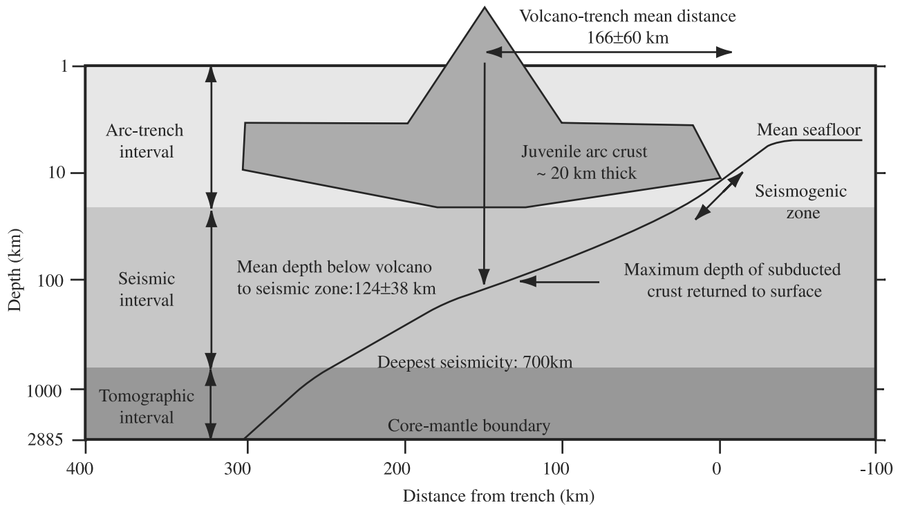
Figure 3. Semilog scale plotting the depth dimension for subduction zones from 1 km below the surface to the core-mantle boundary. Mean depth of ocean (3880 m) is from Kennett [1982]. Typical crustal thickness ( \sim 20 km) for juvenile arc crust is from Suyehiro et al. [1996]; crust associated with Andean-type convergent margins may be up to 70 km thick. Mean distance of arc volcanoes to trench ( 166 \pm 60 km) and of depth beneath arc volcano to seismic zone ( 124 \pm 38 km) are from Gill [1981]. Greatest depth of subducted material returned to surface ( \sim 100 km) is from Ernst [1999]. Note vertical axis encompasses >3 orders of magnitude.
