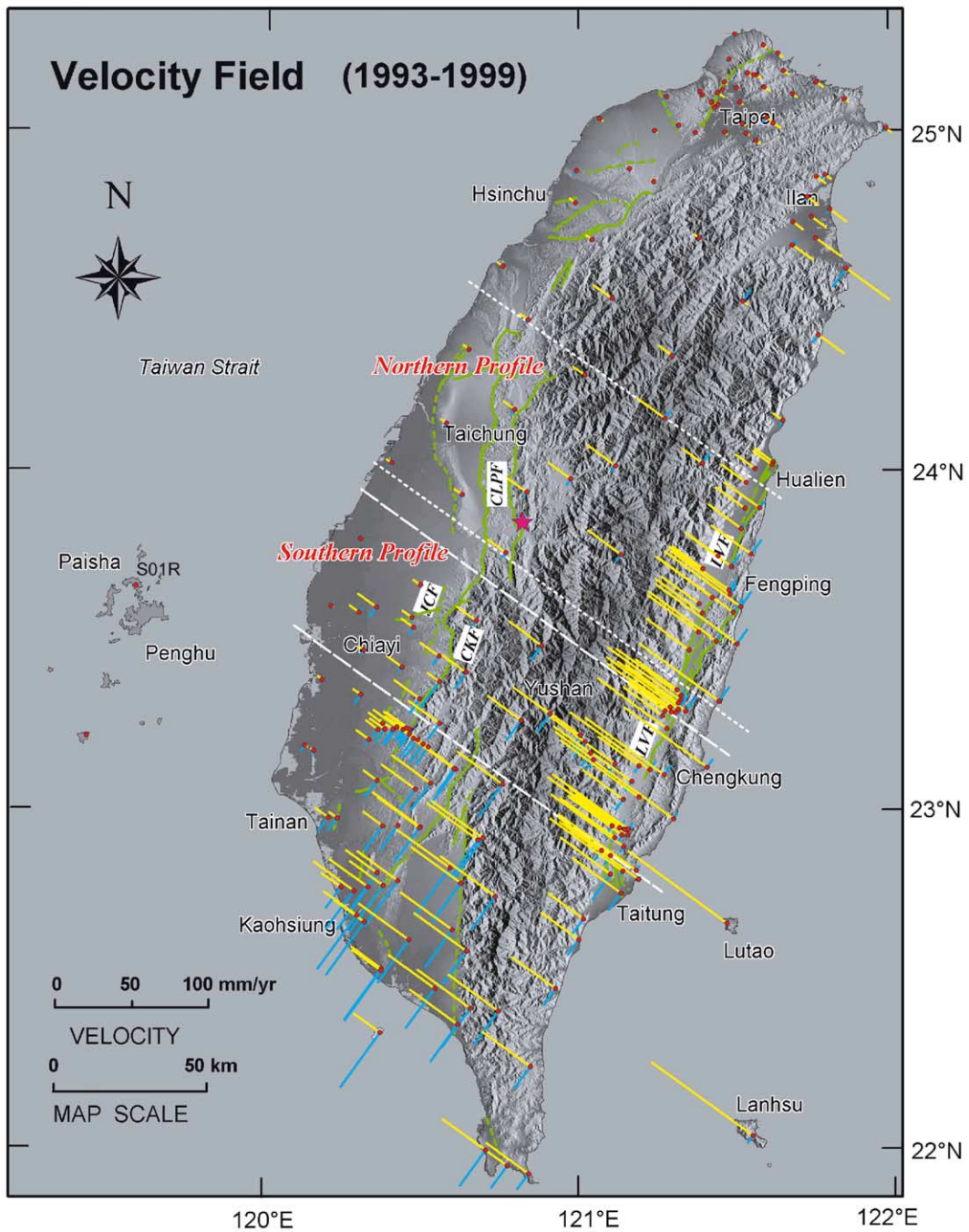
Fig. 1. Shaded relief topographic map of Taiwan. Major faults are indicated as green lines. Red dots correspond to GPS stations, with yellow and blue lines indicating GPS velocities projected parallel and normal to the direction of plate motion. The short-dash and long-dash lines denote the northern and southern sections, respectively. The pink star indicates the epicenter of the Chi-Chi earthquake.
