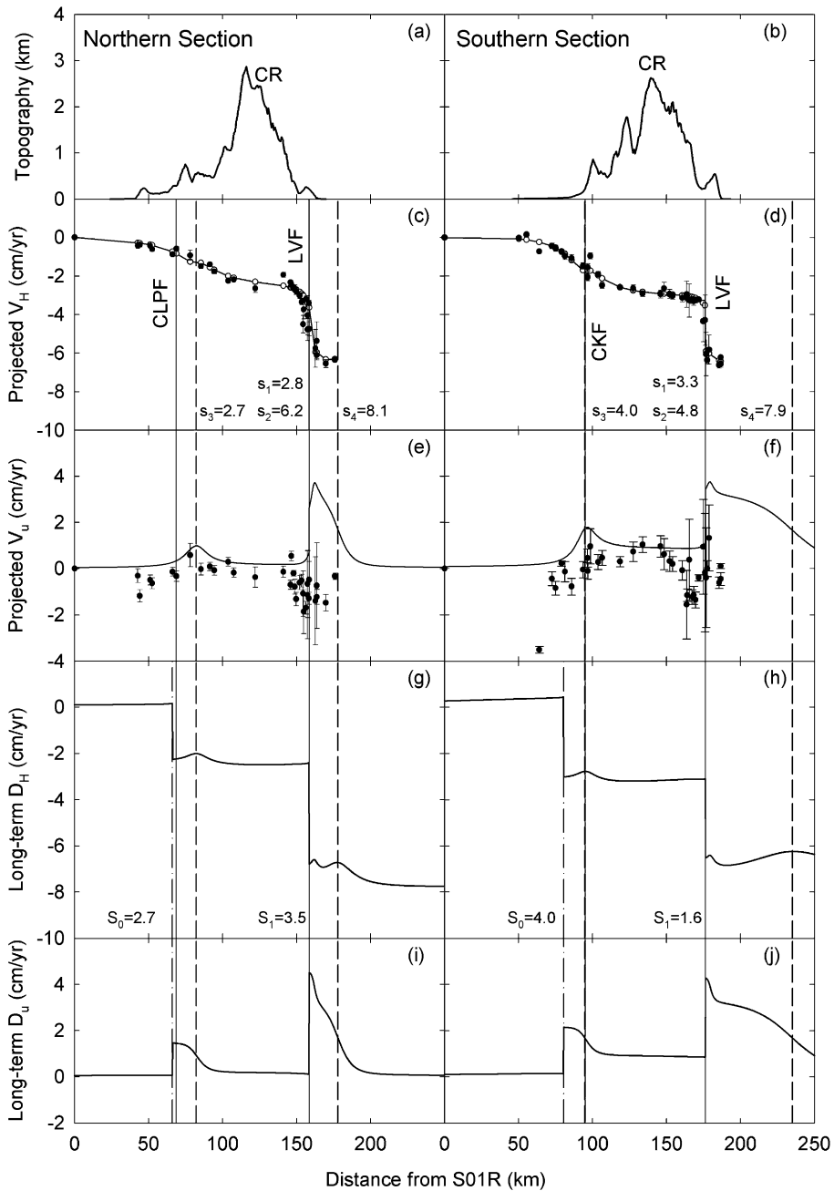
Fig. 3. Comparison of observations and predictions from the best-fit composite dislocation model. The left and right columns correspond to the northern and southern profiles, respectively. (a,b) Topography. (c,d) Horizontal velocities. (e,f) Vertical velocities. Solid circles with error bars are the observed velocities, while the curves with open circles represent the optimal model. S_1 , S_2 , S_3 and S_4 represent slip rates (cm/yr) on each fault patch. CLPF, CKF, and LVF (solid lines) denote the Chelungpu Fault, Chukou Fault and Longitudinal Valley Fault, respectively. Dashed lines represent the location of two patches of buried dislocations. (g,h) Predicted long-term horizontal and (i,j) vertical displacement rates. Dash-dot lines indicate the suggested location ( S_0 ) for a future rupture.
