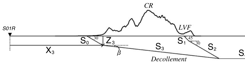
Fig. 2. A schematic of the assumed fault geometry of our two-dimensional interseismic dislocation model. Topography is shown with 6\times vertical exaggeration. S_0 denotes the suggested fault for a future rupture. S_1 and S_2 correspond to two segments of the LVF, while S_3 and S_4 correspond to two segments of the buried dislocations in the west and east of the LVF, respectively. \beta is the dip of S_3 . ( X_3 , Z_3 ) denote the end point of the buried dislocation. CR indicates the Central Range.
